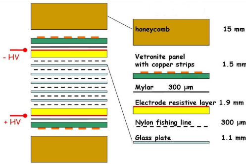
Figure 4: Schematic view of the structure of the MRPC.
