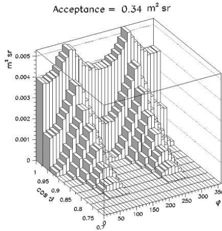
Figure 5: EEE telescope acceptance. The integrated acceptance is 0.34 \text{ m}^2\text{sr} for chambers spaced 1 meter from each other.
