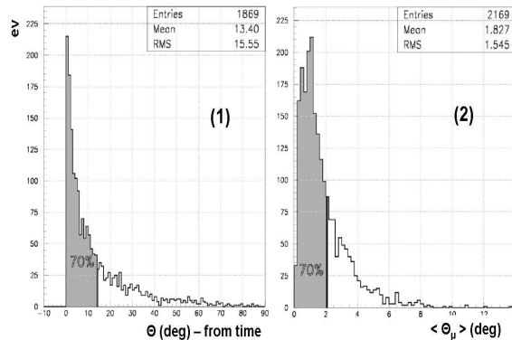
Figure 6: Reconstruction resolution of shower axis direction (see the text).
